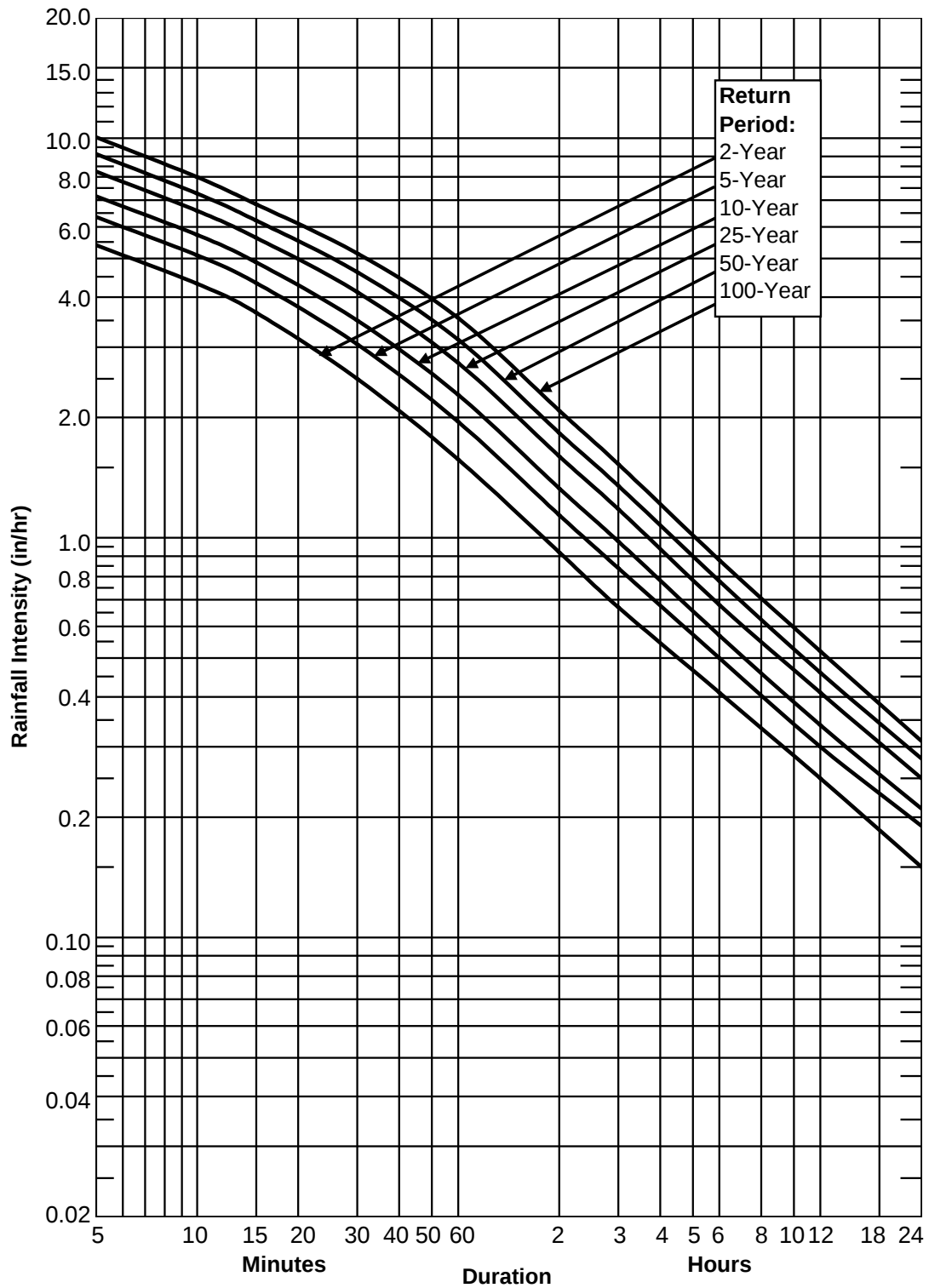
Figure 4A-4 Cookeville IDF Curve
