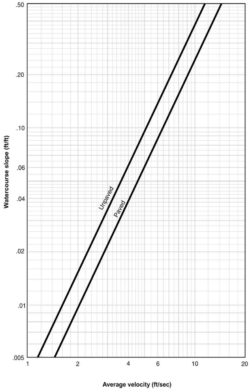
Figure 4A-12 Shallow Concentrated Flow Average Velocities Reference: USDA, Urban Hydrology for Small Watersheds (1986)
