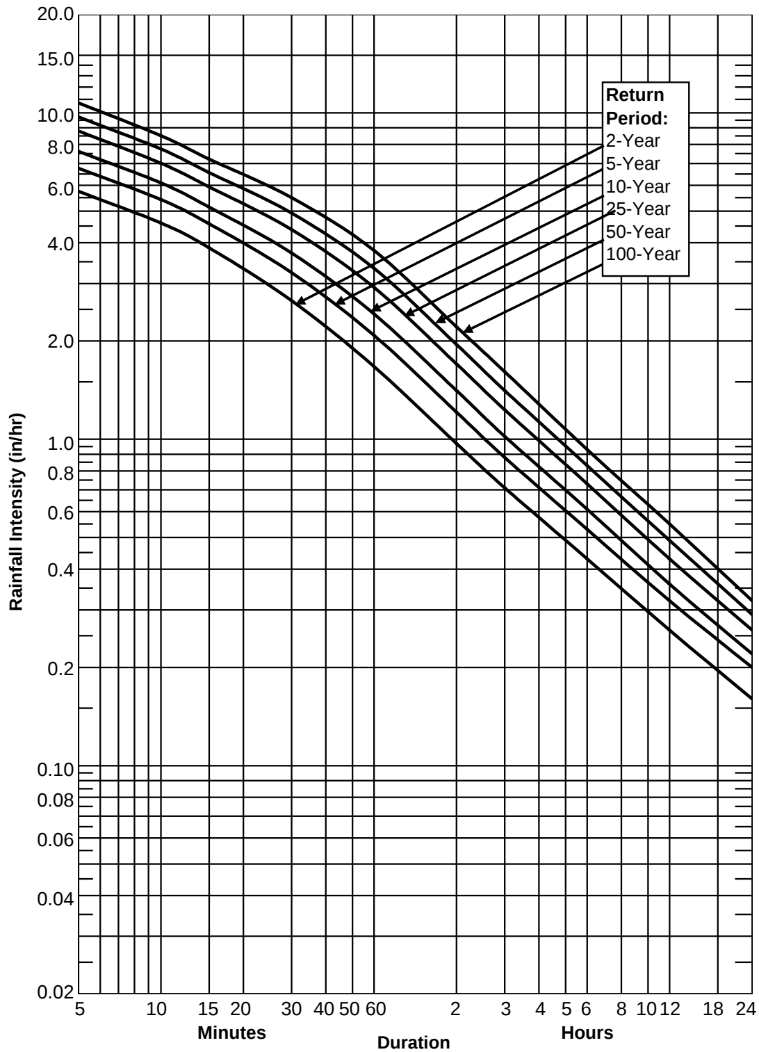
Figure 4A-11 Shelbyville IDF Curve
