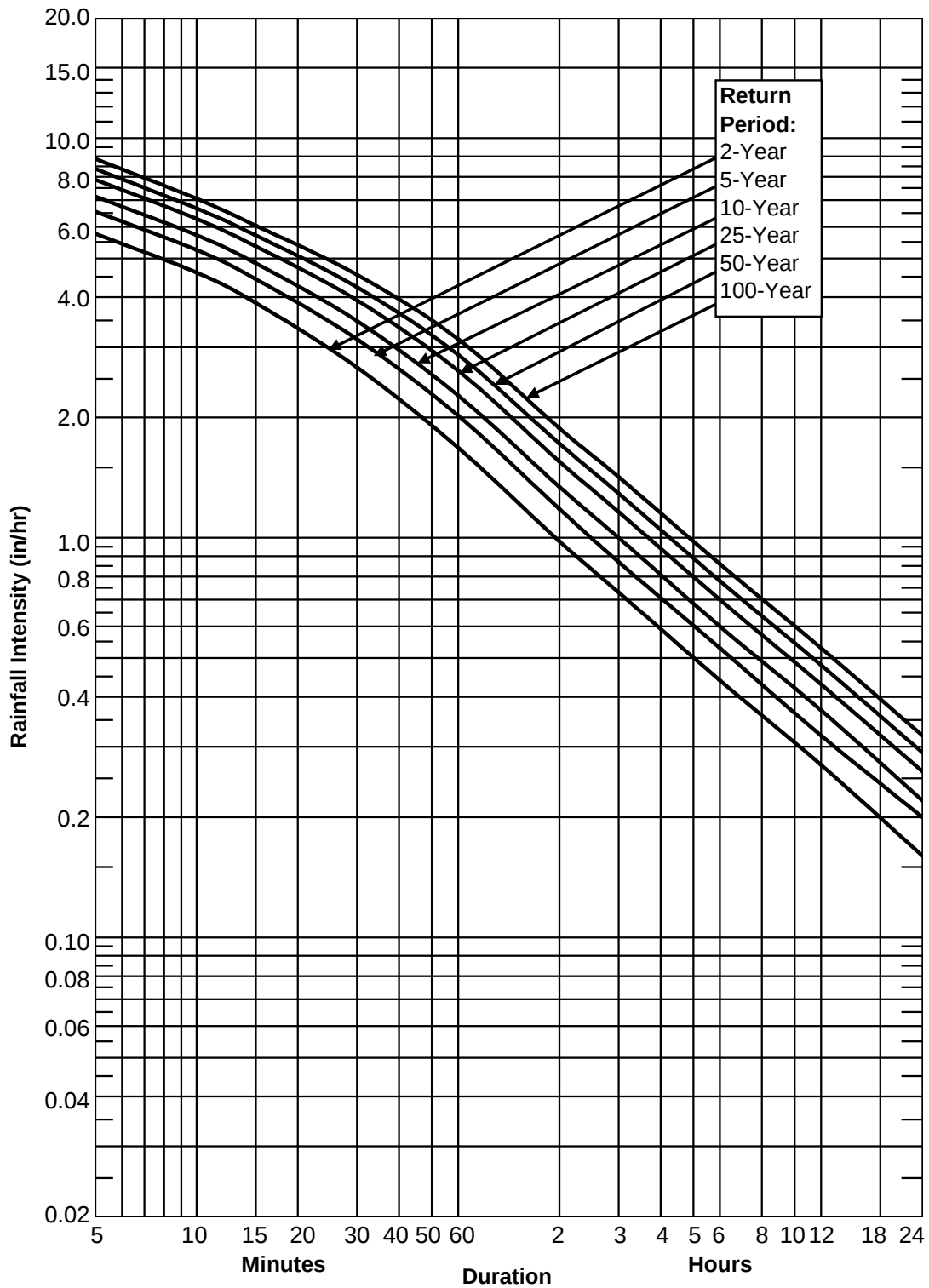
Figure 4A-5 Jackson IDF Curve
