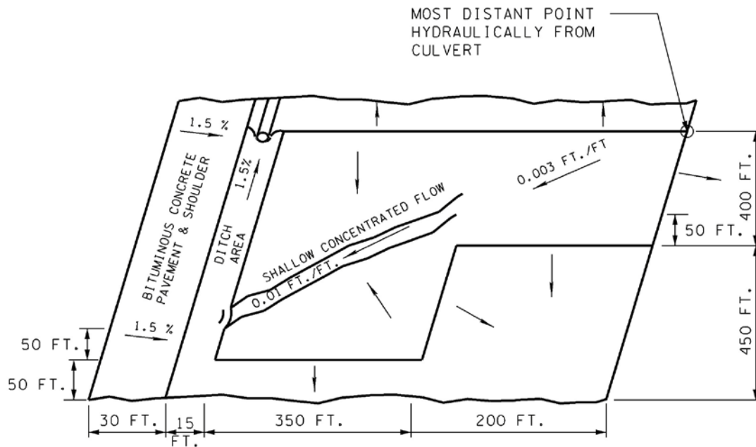
Figure 4A-19 Complex Drainage Area Example
