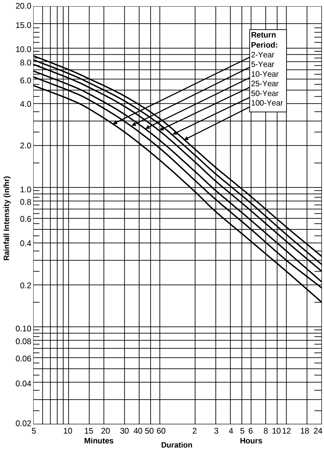
Figure 4A-3 Clarksville IDF Curve
