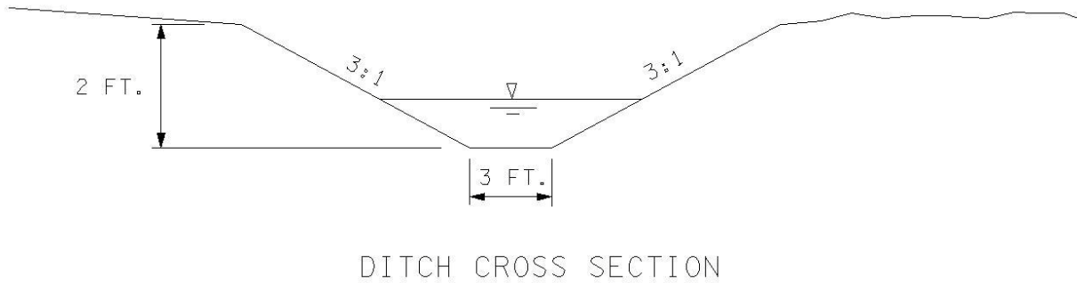
Figure 4A-18 Ditch Cross Section for Simple Drainage Area Example
