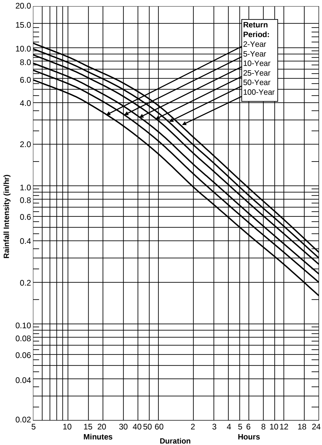
Figure 4A-8 Lawrenceburg IDF Curve NOTE: T_c = 5 minutes is a minimum value to use in all cases Reference: National Weather Service, NOAA Atlas 14, Volume 2 (2004)
