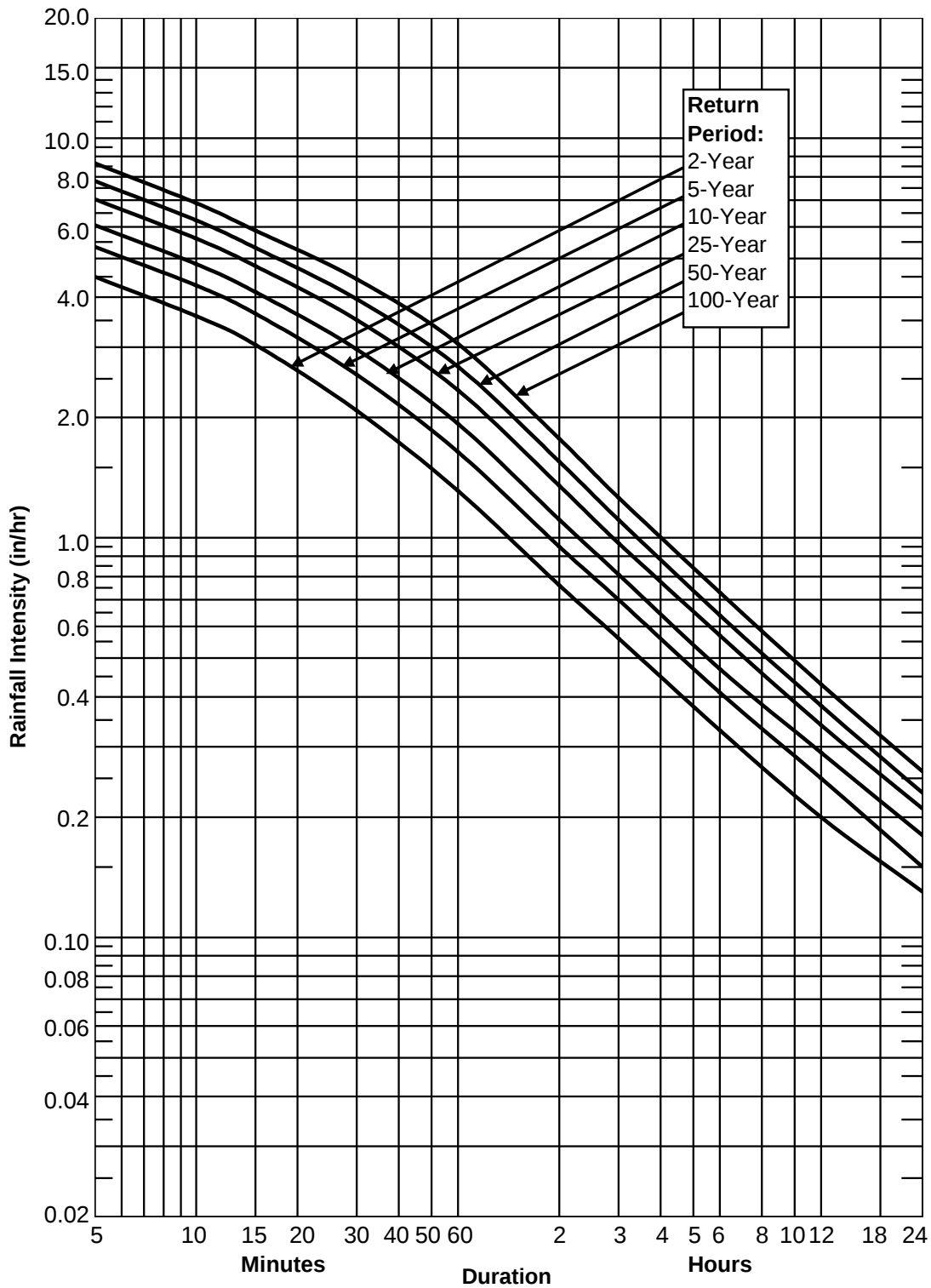
Figure 4A-7 Knoxville IDF Curve
