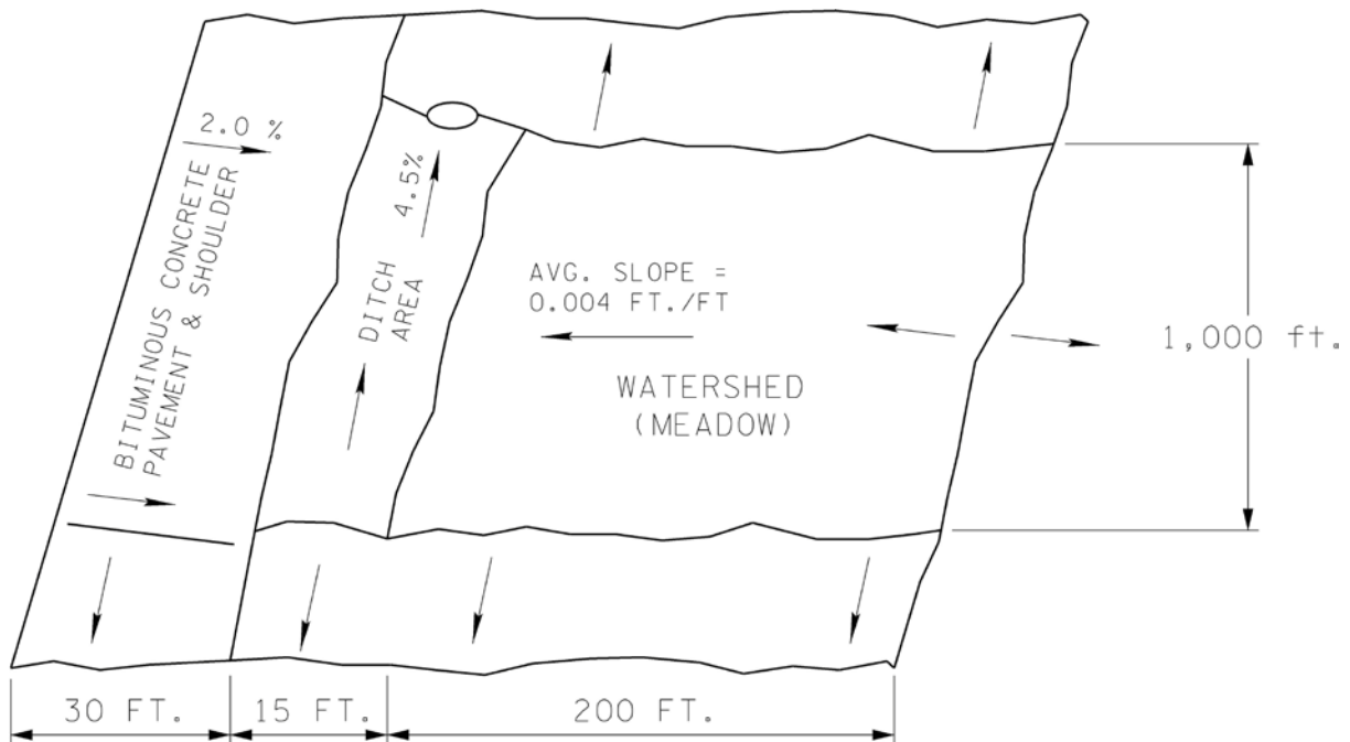
Figure 4A-17 Simple Drainage Area Example
