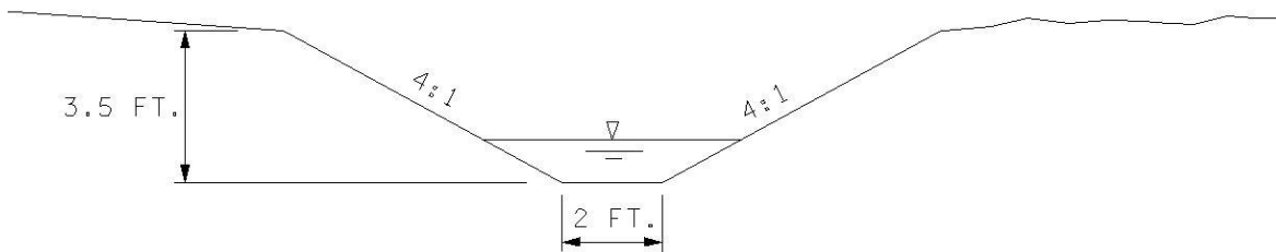
DITCH CROSS SECTION
