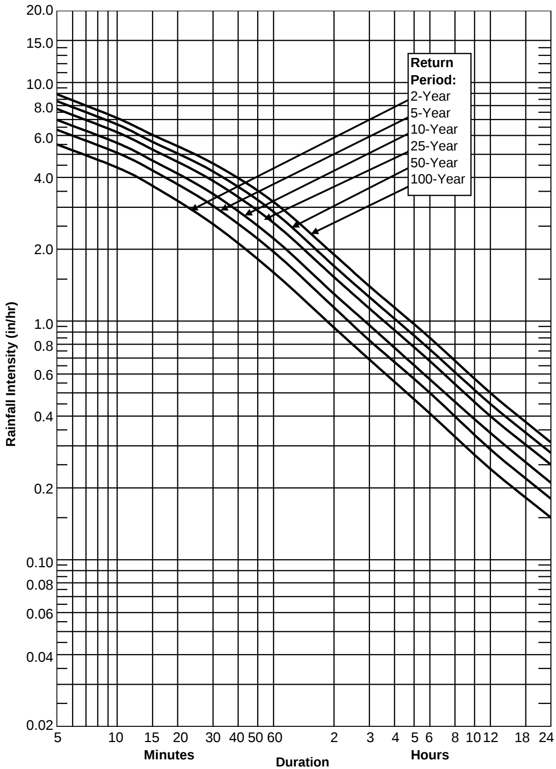
Figure 4A-9 Lebanon IDF Curve
